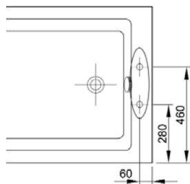
Bath Filler 2 Holes / İki Delikli Batarya
