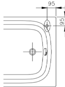
Bath Filler one Hole / Tek Delikli Batarya
