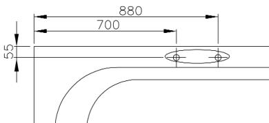
Bath Filler 2 Holes / İki Delikli Batarya
